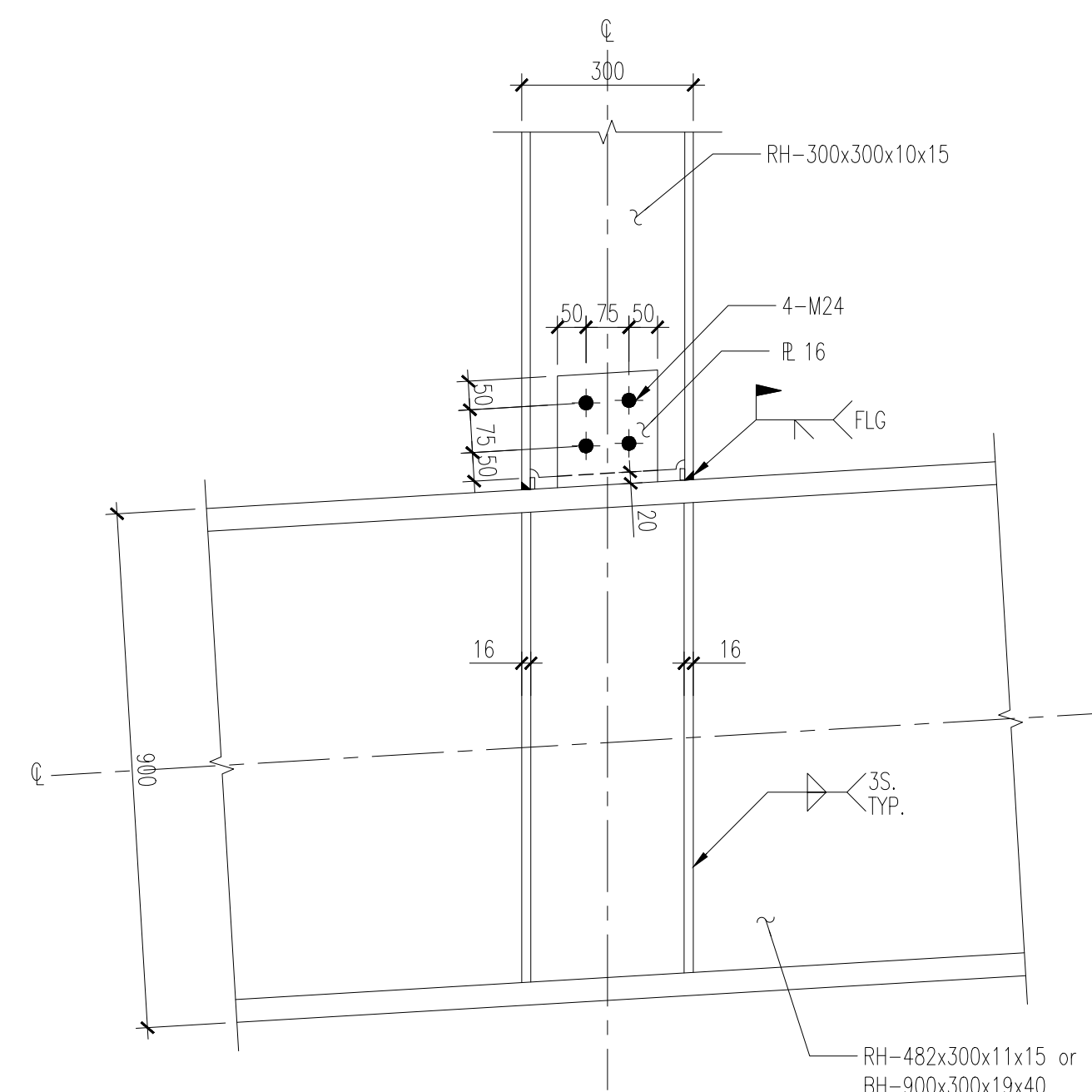
6A RH-300x300柱底接合詳圖 S9-22 S:1/10
