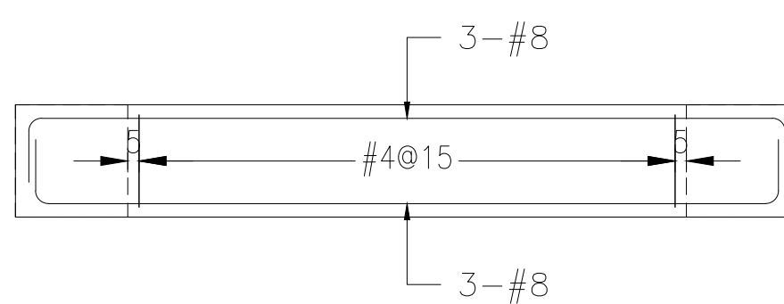
2F B153 (30x50)
