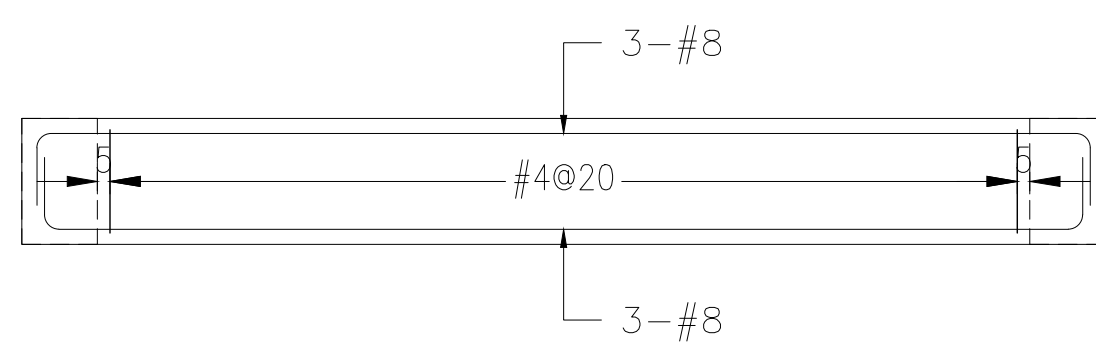
2F bG159 (30x50)
