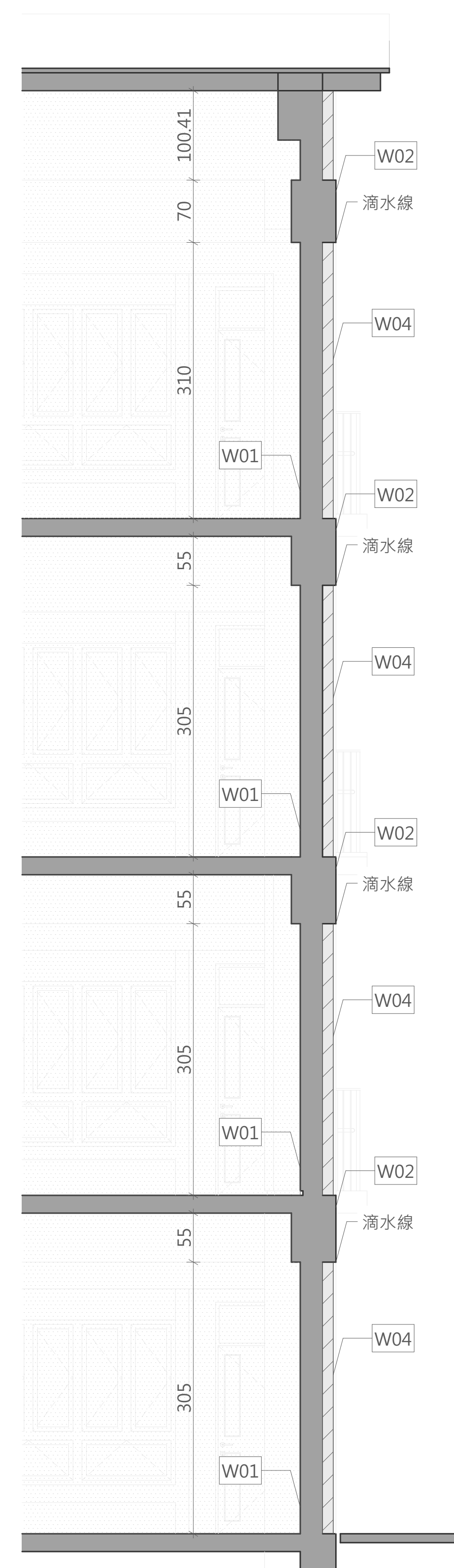
A棟 外牆剖面b A1SCALE=1/40 A3SCALE=1/80
