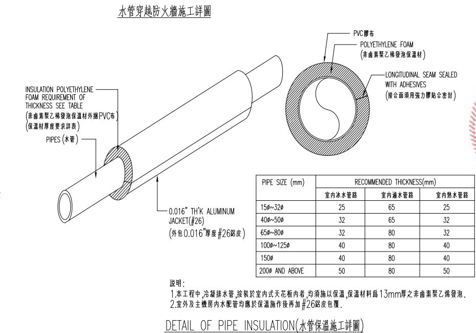
DETAIL OF PIPE INSULATION(水管保溫施工詳圖)
