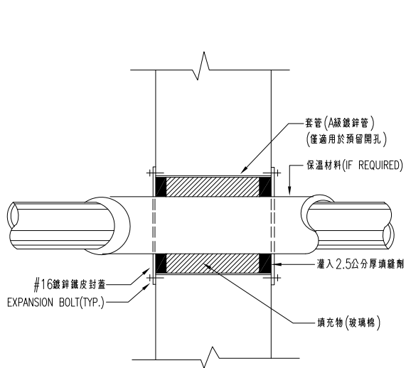
PIPE THROUGH WALL 水管貫穿牆壁詳細圖
