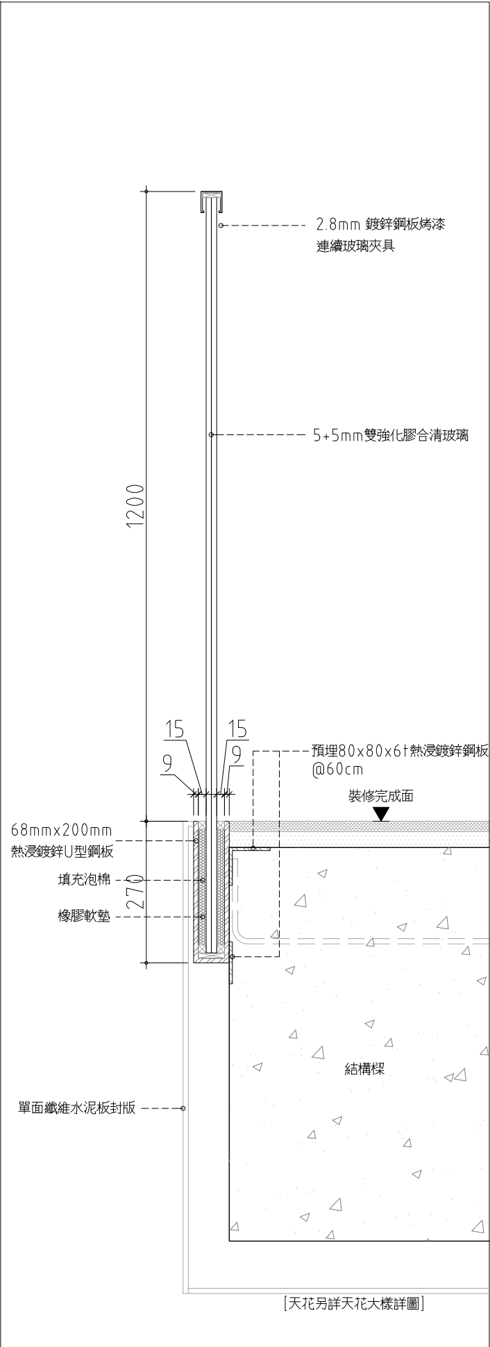
3 玻璃欄杆 typeC 詳圖 SCALE:(A1)1:5 (A3)1:10 UNIT: mm
