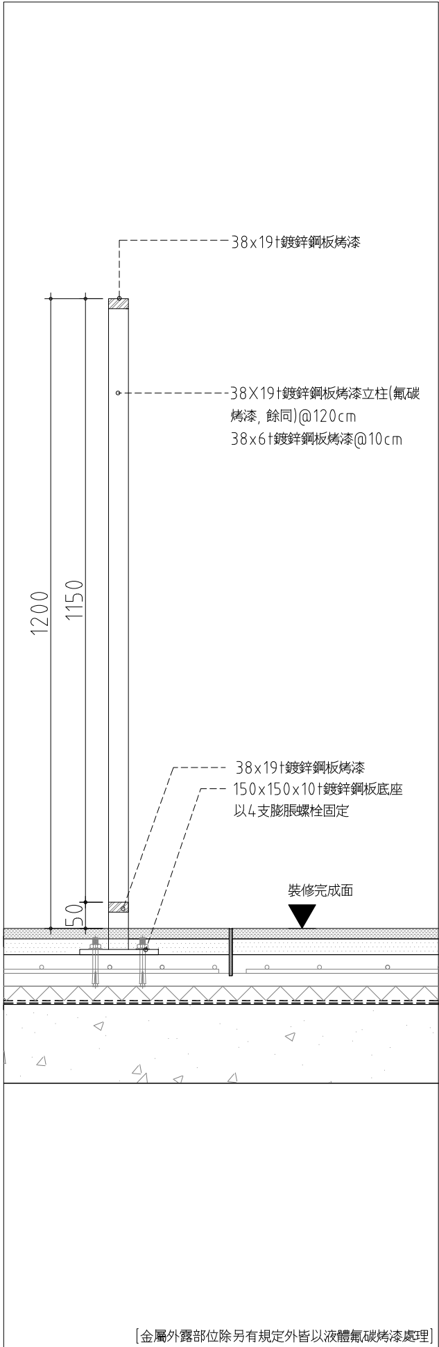
1 金屬欄杆 typeB 詳圖 SCALE:(A1)1:5 (A3)1:10 UNIT: mm
