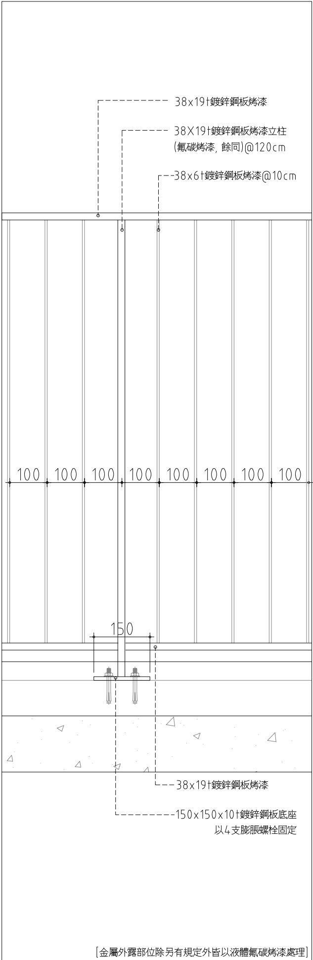
2 金屬欄杆 typeB 詳圖 SCALE:(A1)1:5 (A3)1:10 UNIT: mm
