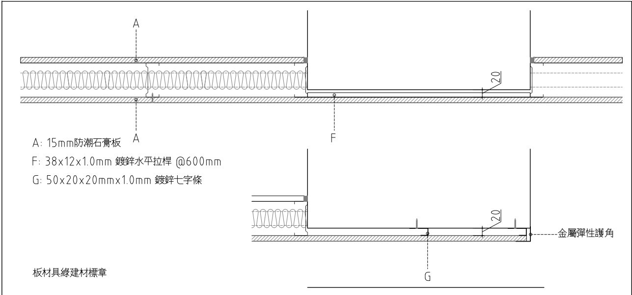
6 TYPE F: 乾式過柱封板 SCALE: 1:5 UNIT: mm
