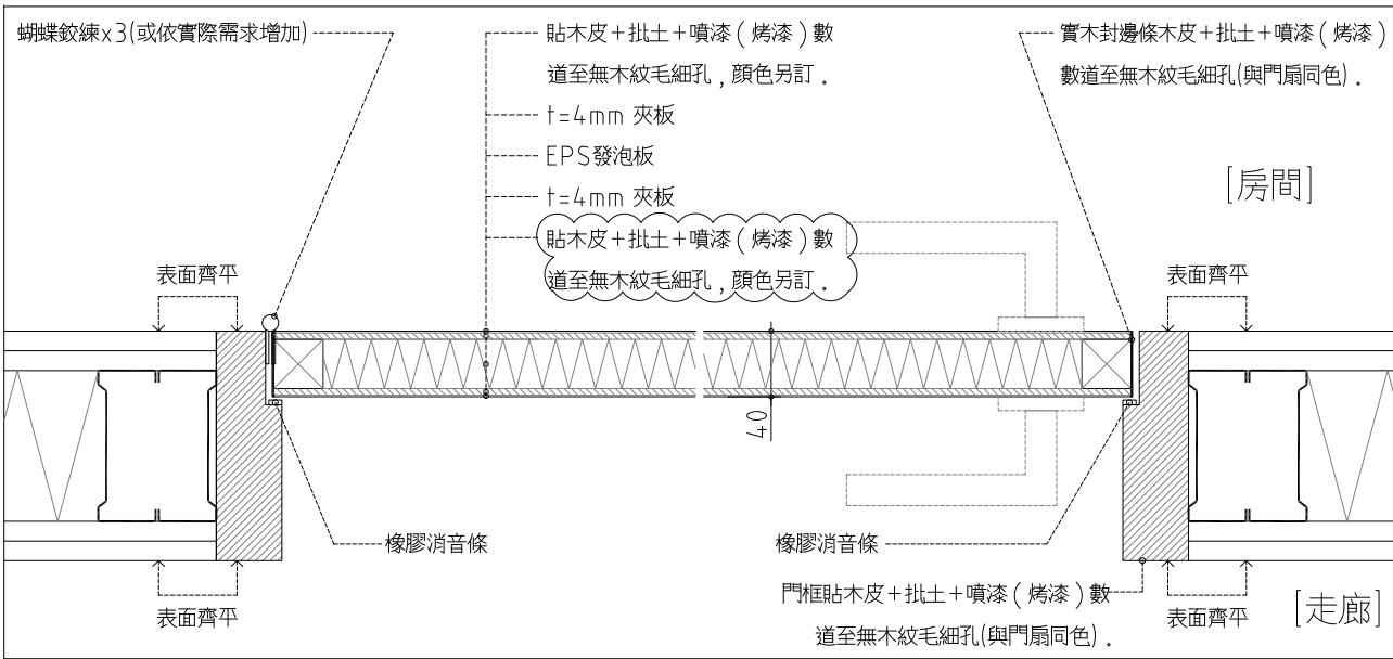
2 EPS木烤漆門 (TYPE A) 細部詳圖 SCALE: 1:2.5 UNIT: mm
