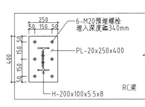
sec B-B
