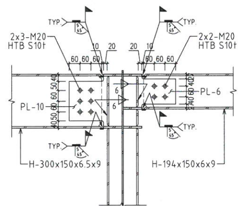
sec B-B
