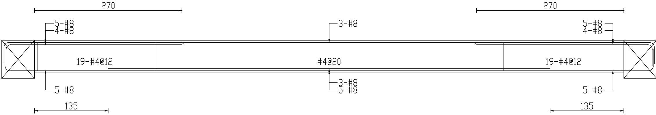
R2F b2(40x60)
