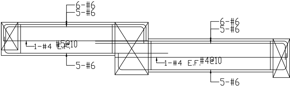
R1F b2(40x60)
