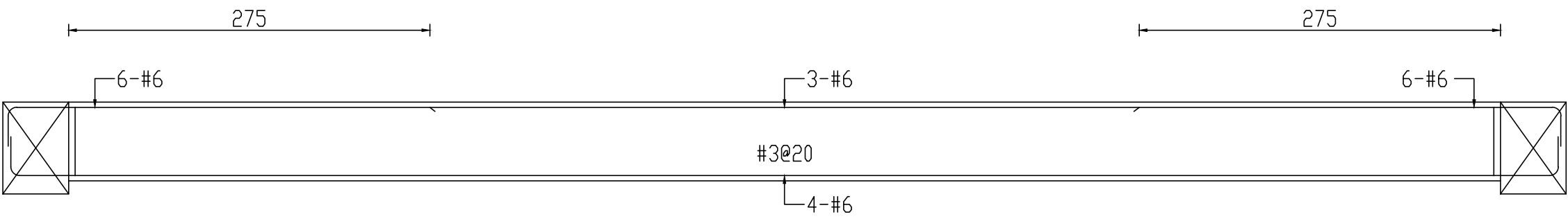
PF b2(40x60)
