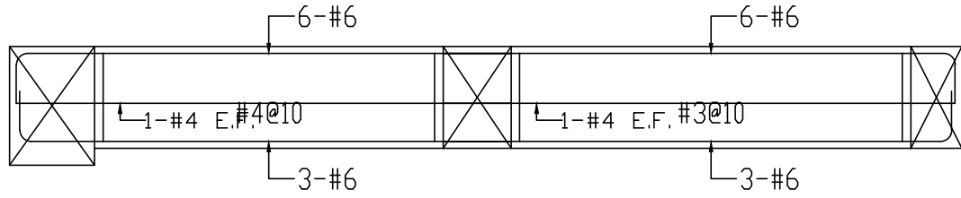
1F b1(40x60)
