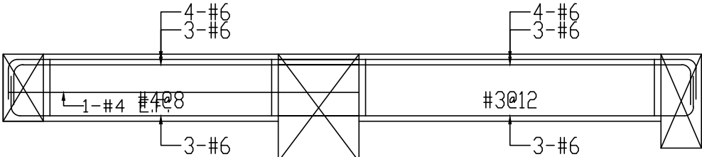
4F b2(30x50)
