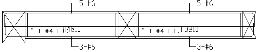
B2F b1(40x60)
