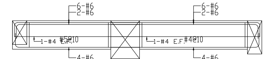
2F b2(40x60)
