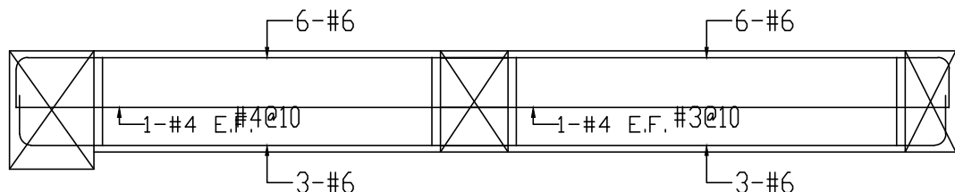
B1F b1(40x60)
