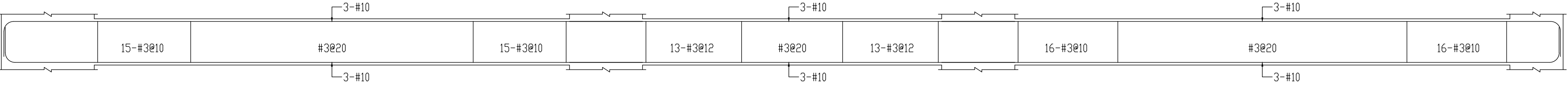
B1F G49(50x70)
