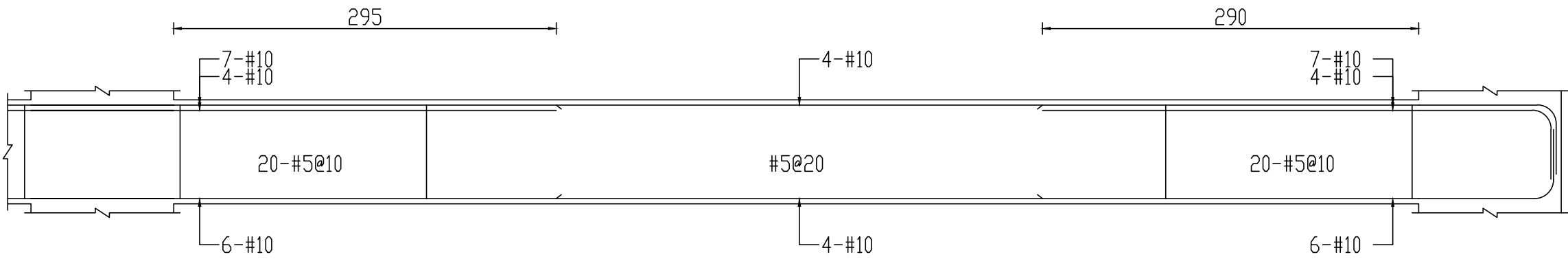
3F B12A(60x80)
