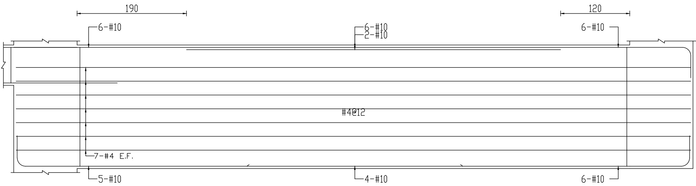
1F FB12A(50x215)
