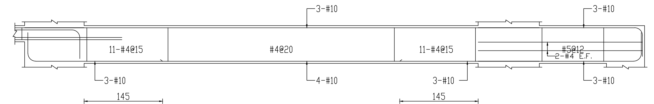
B1F B11(50x70)
