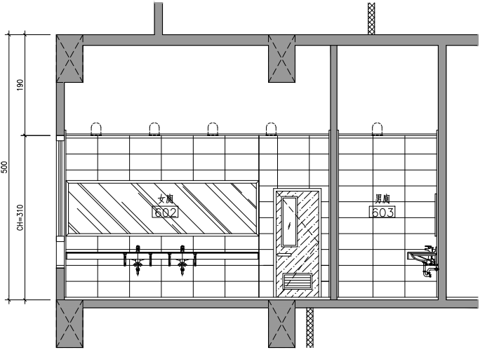
4 A5-48 陸層餐廳廁所剖面詳圖B S:1/50
