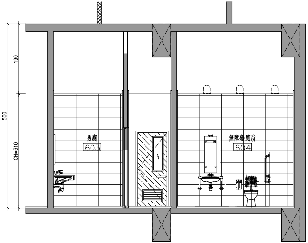
5 A5-48 陸層餐廳廁所剖面詳圖C S:1/50
