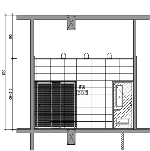
5 A5-48 陸層餐廳廁所剖面詳圖C S:1/50
