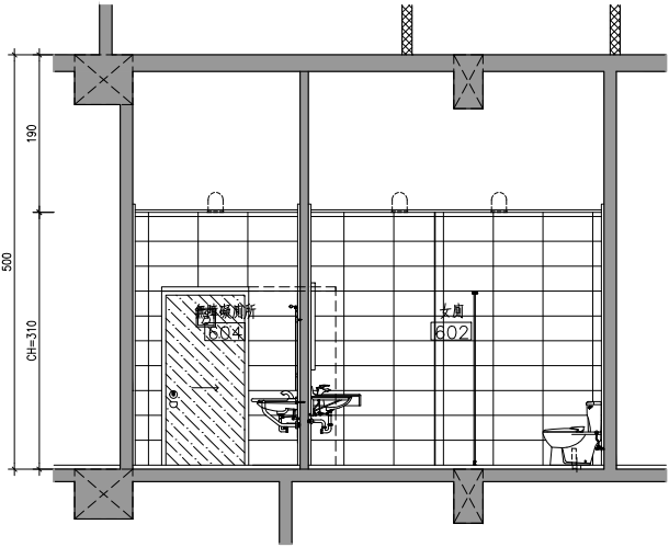
4 A5-48 陸層餐廳廁所剖面詳圖B S:1/50
