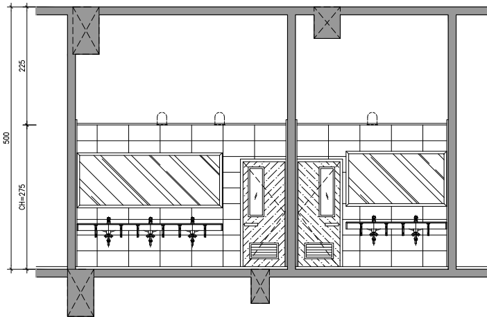
8 貳層補習班廁所剖面詳圖F S:1/50
